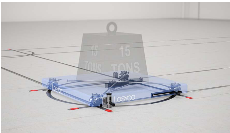
Caption: The next-generation AllRounder transport platform features semi-automatic steering for easy direction changes on intra-logistics rails
